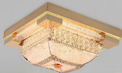
Item: TM-570 Size: Ø260mm Lamp: LED 18W Con 3 cambios calida / bca / intermedia Outside Color 4000K
